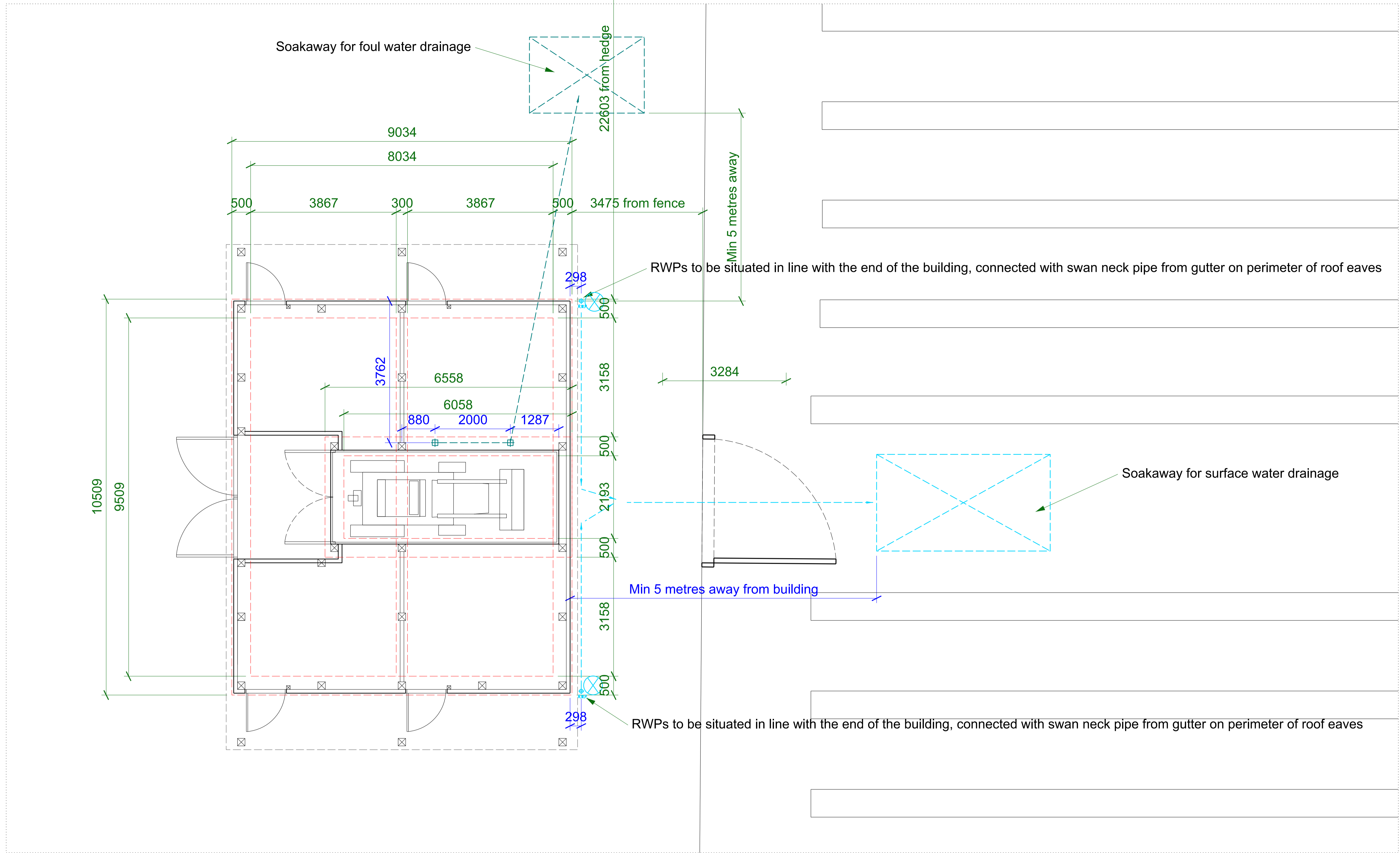
Proposed Ground Floor Plan
